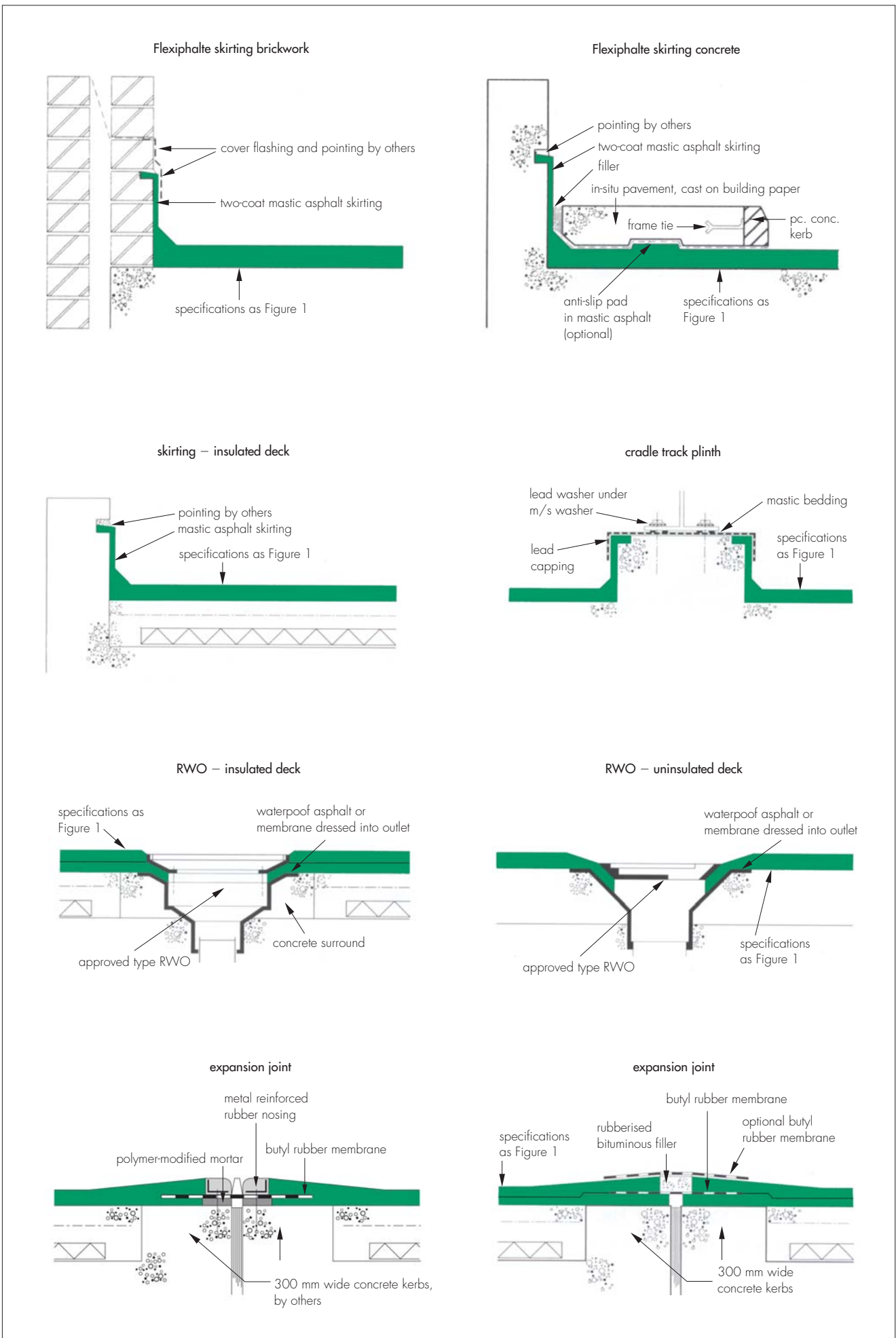
Figure 2 Typical installation details
